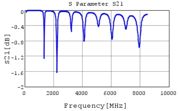
GQM2195C2E151GB12 S21 DCOV, 25degC
