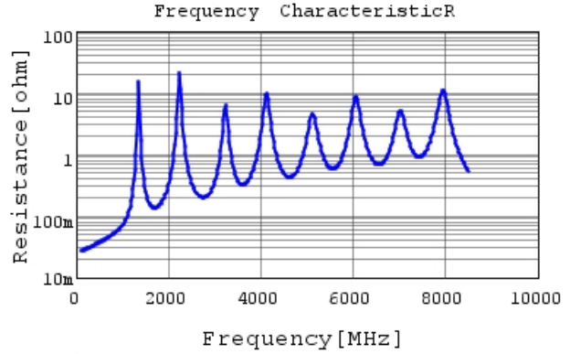
GQM2195C2E151GB12 R DC0V, 25degC
