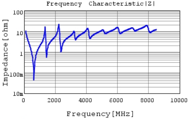
GQM2195C2E151GB12 |Z| DC0V, 25degC
