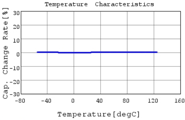
GQM2195C2E151GB12 C-Temp. capchange, DCOV, 1
