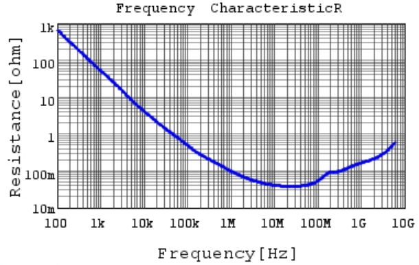
GRM033B31A223ME84 R DCOV, 20degC
