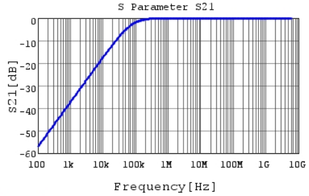
GRM033B31A223ME84 S21 DC0V, 20degC
