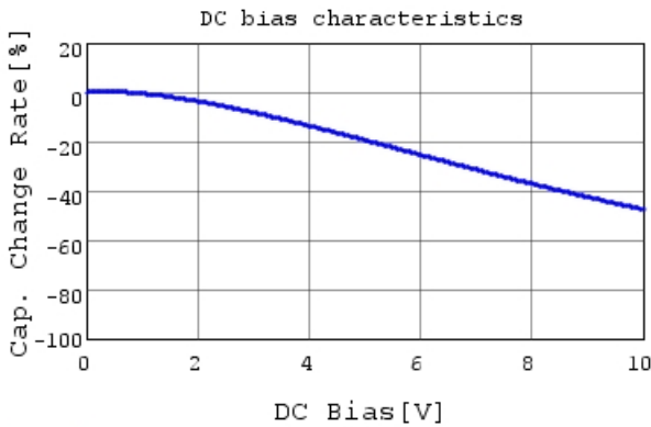
GRM033B31A223ME84 C-DC bias capchange, 20.0c
