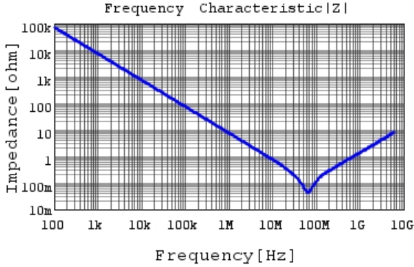
GRM033B31A223ME84 |Z| DCOV, 20degC
