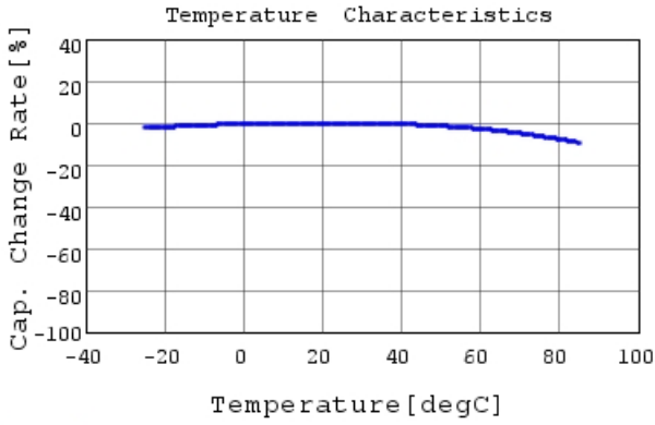
GRM033B31A223ME84 C-Temp. capchange, DC0.0V,
