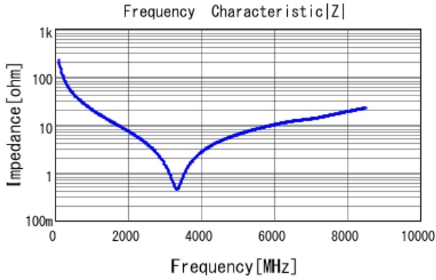
GRM1555C1H7R0BA01 |Z| DCOV, 25degC
