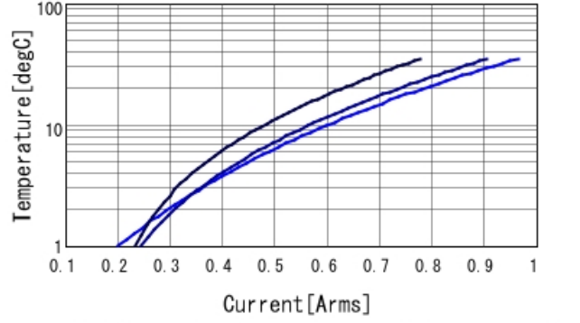
Temp. Rise from ripple Characteristics
