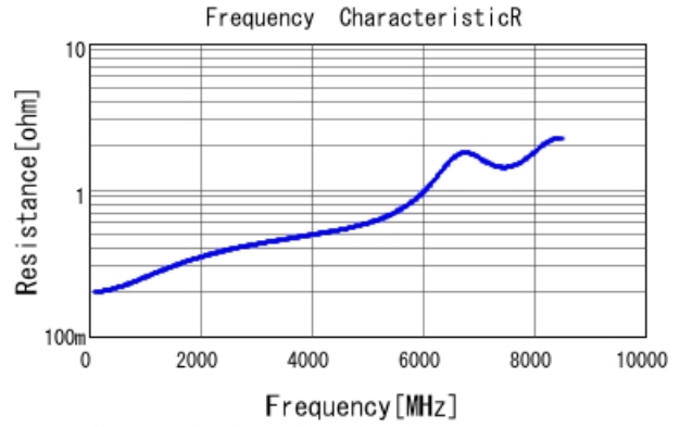
GRM1555C1H7R0BA01 R DCOV, 25degC
