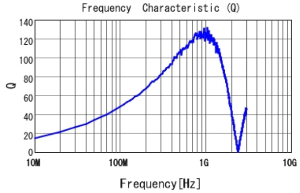
LQW2UAS33NG00 Q
