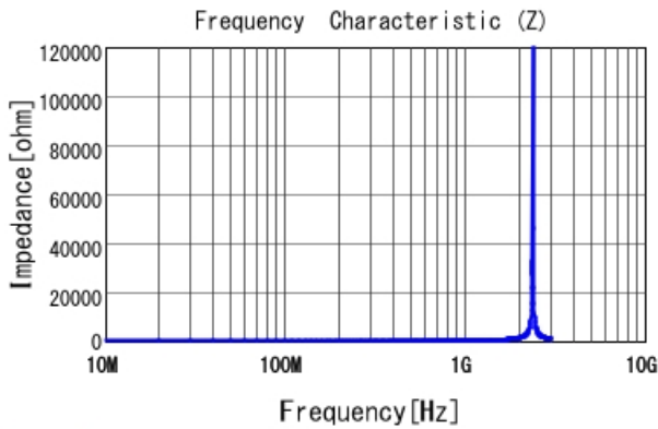
LQW2UAS33NG00 |Z|
