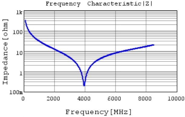
GCQ1555C1H4R8BB01 |Z| DC0V, 25degC
