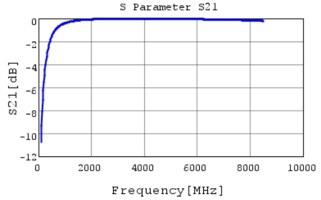
GCQ1555C1H4R8BB01 S21 DCOV, 25degC
