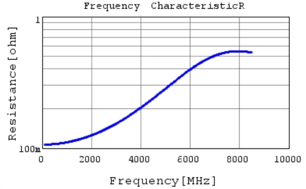
GCQ1555C1H4R8BB01 R DC0V, 25degC
