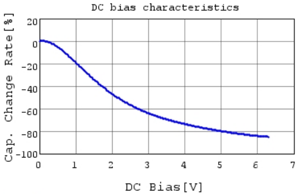
GRM022R60J224ME14 C-DC bias capchange, 25.0c
