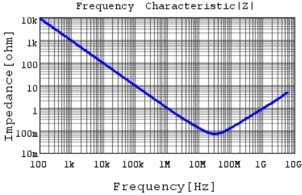
GRM022R60J224ME14 |Z| DCOV, 25degC
