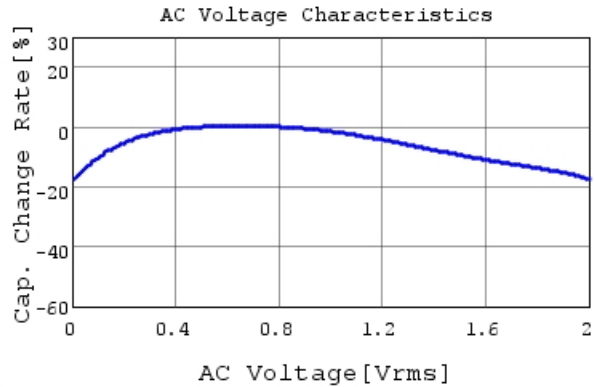
GRM022R60J224ME14 C-AC Voltage capchange, Dc
