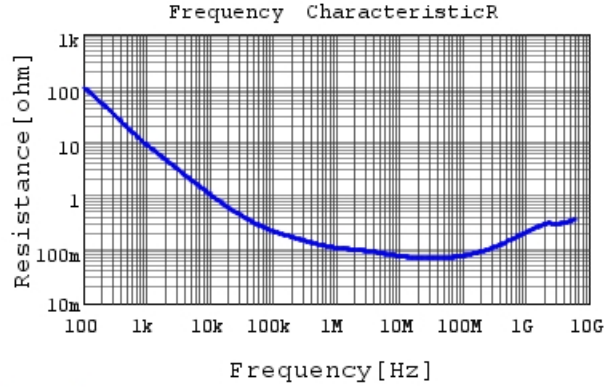
GRM022R60J224ME14 R DCOV, 25degC
