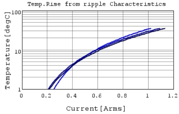
GRM022R60J224ME14 Temp.rise — 300kHz
