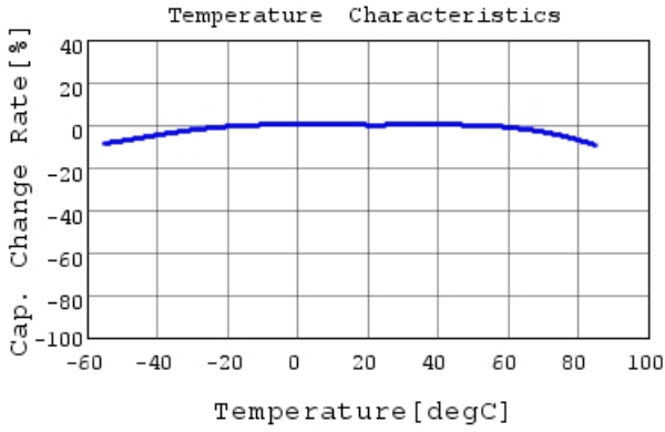
GRM022R60J224ME14 C-Temp. capchange, DC0.0V,
