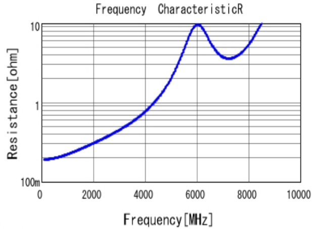
■ GRM1552C1H9R0DA01 R DCOV, 20degC
