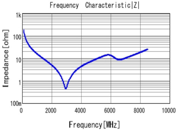
■ GRM1552C1H9R0DA01 |Z| DCOV, 20degC
