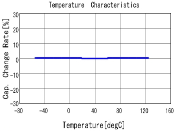
■ GRM1552C1H9R0DA01 C-Temp. capchange, DCOV, AC1Vrms
