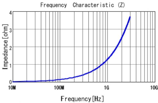
LQP02TQ0N2B02 |Z|
