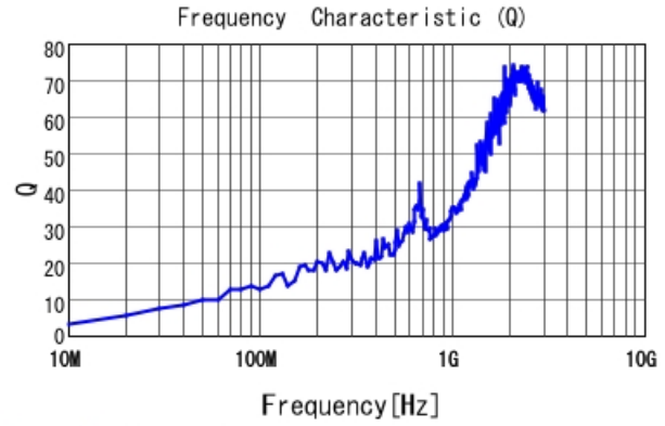
LQP02TQ0N2B02 Q
