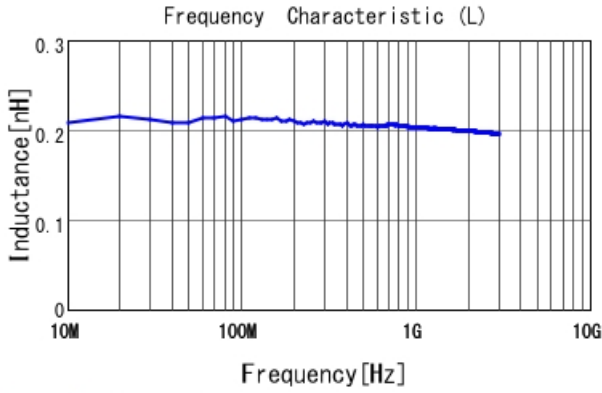
LQP02TQ0N2B02 L
