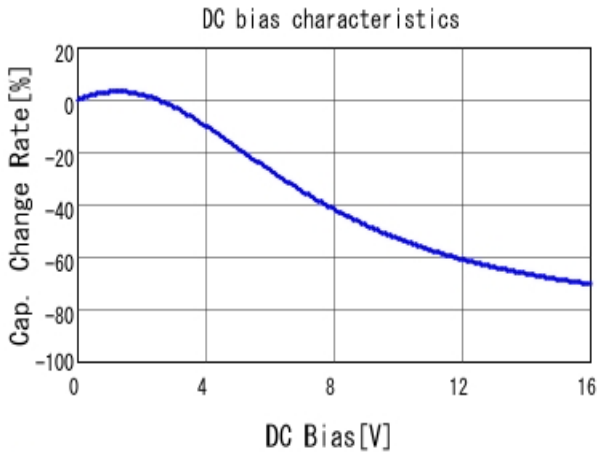
■ GRJ32ER71C226KE11 C-DC bias capchange, 25.0degC, ACO.
