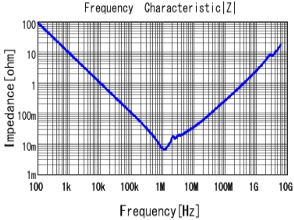
■ GRJ32ER71C226KE11 |Z| DCOV, 25degC
