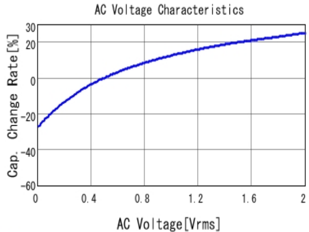
■ GRJ32ER71C226KE11 C-AC Voltage capchange, DCOV, 25.0d
