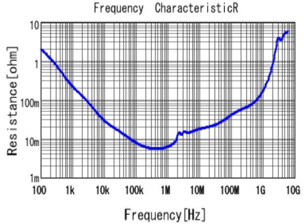
■ GRJ32ER71C226KE11 R DCOV, 25degC
