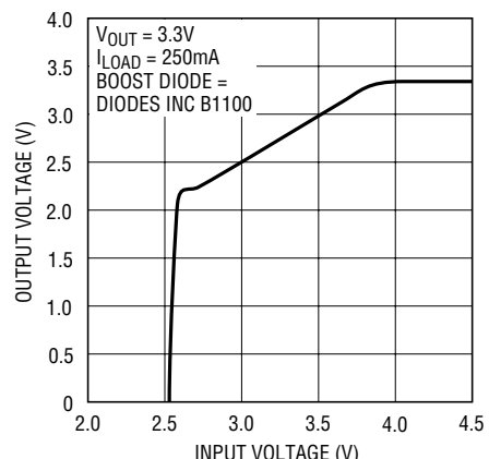
Dropout Operation
