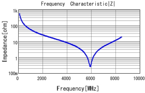
GJM0335C1E2R8BB01 |Z| DCOV, 25degC
