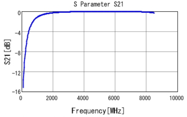
GJM0335C1E2R8BB01 S21 DC0V, 25degC
