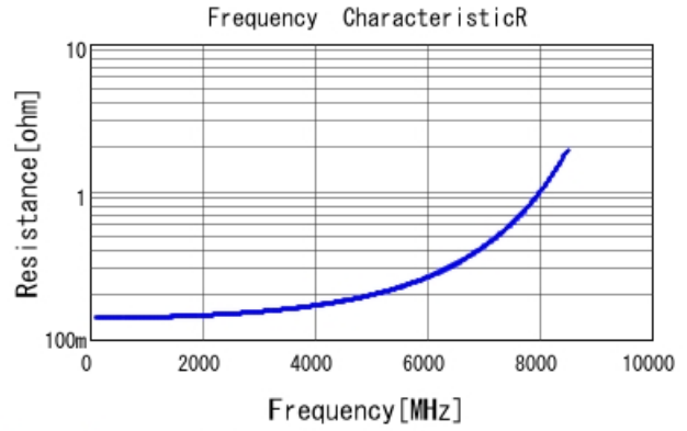
GJM0335C1E2R8BB01 R DCOV, 25degC
