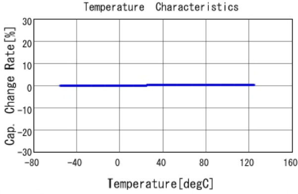
GJM0335C1E2R8BB01 C-Temp. capchange, DC0V, AC1Vrms
