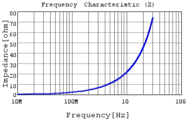
LQG15HN3N6S02 |Z|
