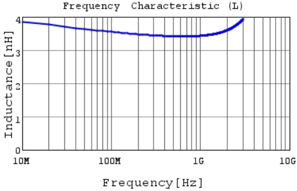
LQG15HN3N6S02 L
