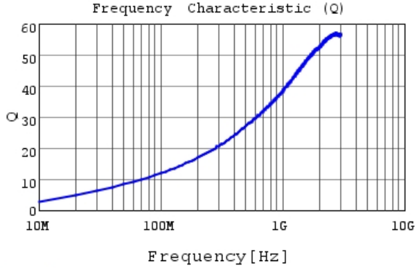
LQG15HN3N6S02 Q
