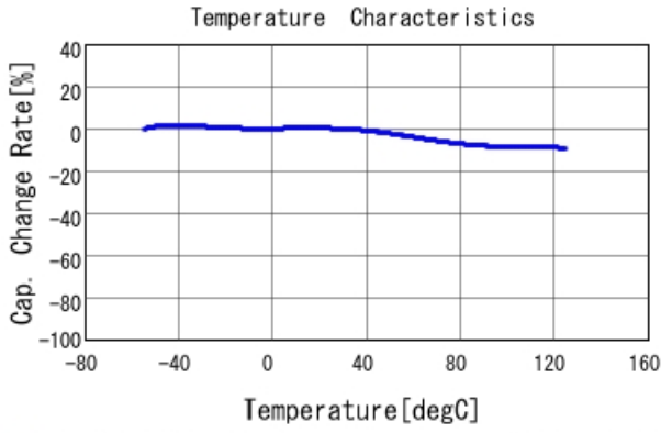
■ GCD188R71H102KA01 C-Temp. capchange, DCO. 0V, AC1. 0Vrm
