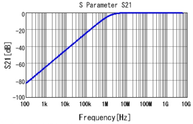
■ GCD188R71H102KA01 S21 DCOV, 25degC
