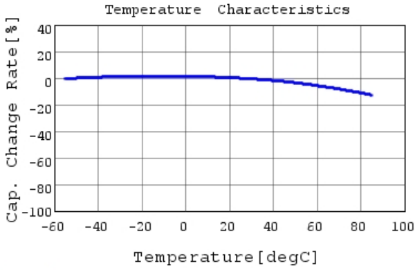
GRM033R61C273KE84 C-Temp. capchange, DC0.0V,
