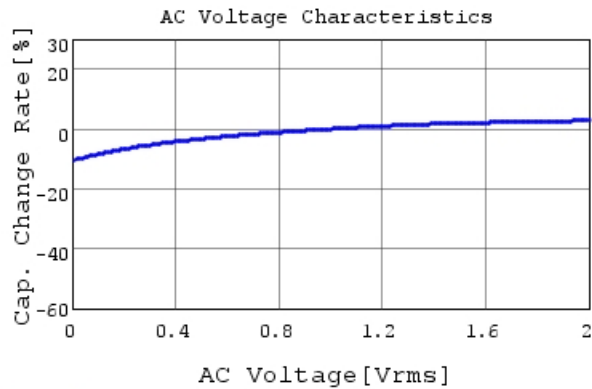
GRM033R61C273KE84 C-AC Voltage capchange, Dc
