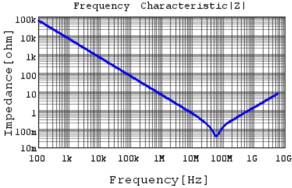
GRM033R61C273KE84 |Z| DCOV, 25degC
