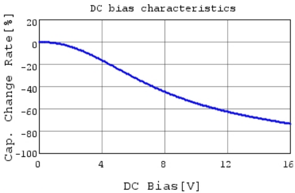
GRM033R61C273KE84 C-DC bias capchange, 25.0c
