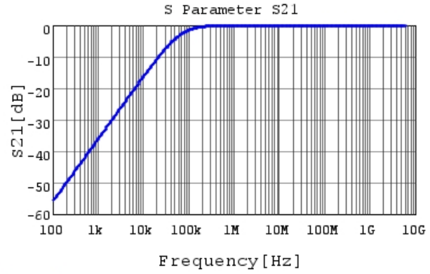
GRM033R61C273KE84 S21 DC0V,25degC
