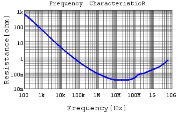
GRM033R61C273KE84 R DCOV, 25degC
