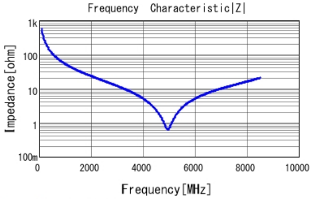
GRM1555C1H2R9WA01 |Z| DCOV, 25degC
