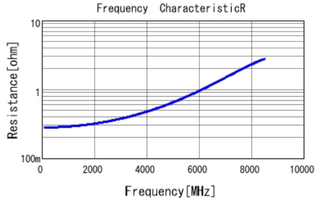
GRM1555C1H2R9WA01 R DCOV, 25degC
