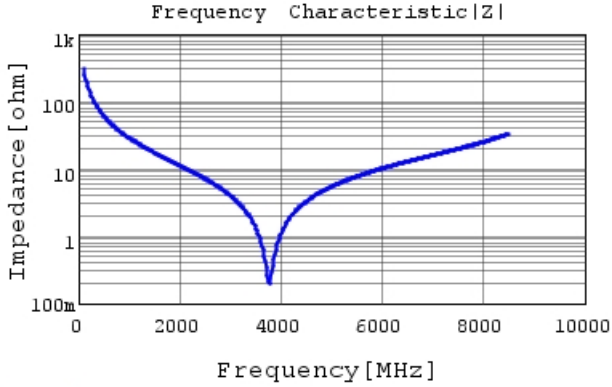
GCQ1555C1H5R2BB01 |Z| DC0V, 25degC
