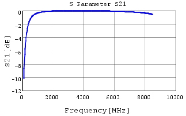
GCQ1555C1H5R2BB01 S21 DCOV, 25degC
