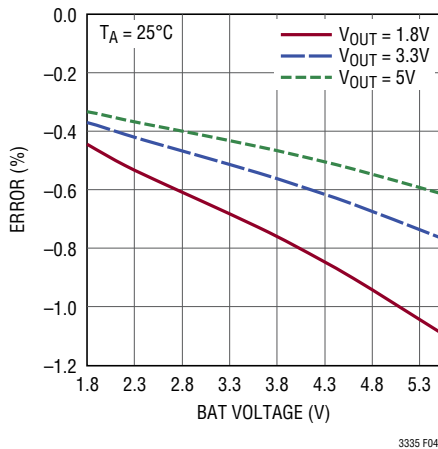
Figure 4. Typical Error Due to Input Quiescent Current for 250mA I_{PEAK} Setting
