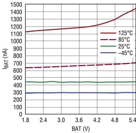
Input Quiescent Current in Shutdown vs BAT
