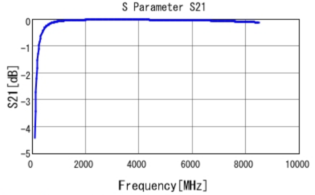
GRM0225C1E120GA03 S21 DCOV, 25degC
