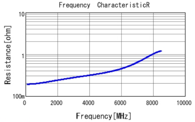
GRM0225C1E120GA03 R DCOV, 25degC
