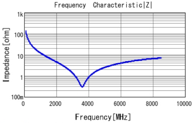
GRM0225C1E120GA03 |Z| DCOV, 25degC
