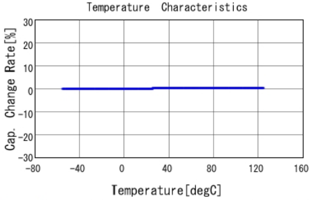
GRM0225C1E120GA03 C-Temp. capchange, DCOV, AC1Vrms
