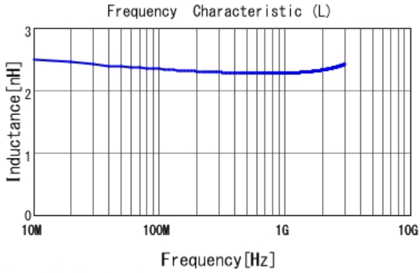
LQP03HQ2N3B02 L
