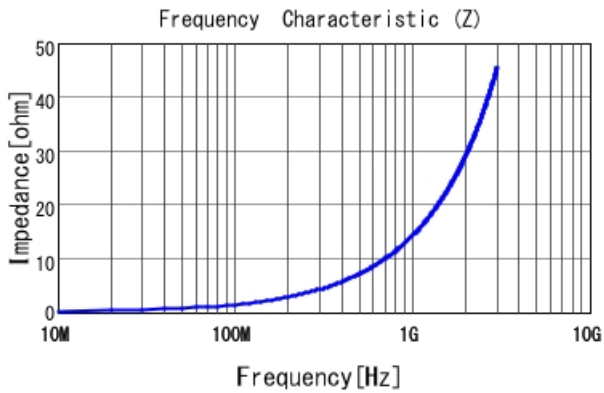
LQP03HQ2N3B02 |Z|
