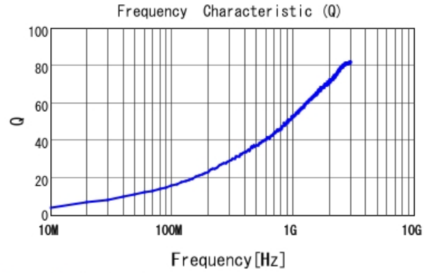
LQP03HQ2N3B02 Q
