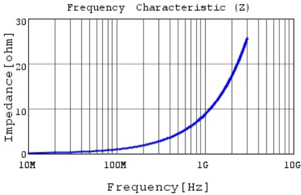
LQP02HQ1N4B02 |Z|
