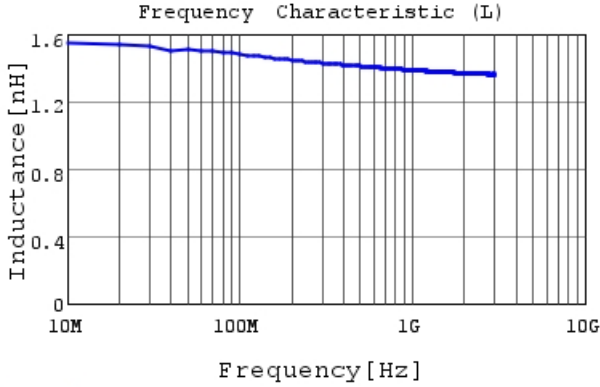
LQP02HQ1N4B02 L
