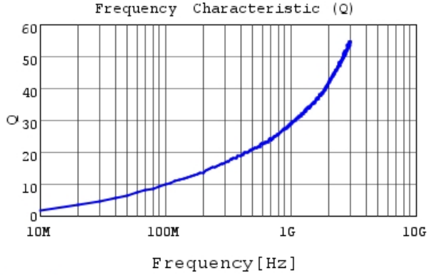
LQP02HQ1N4B02 Q
