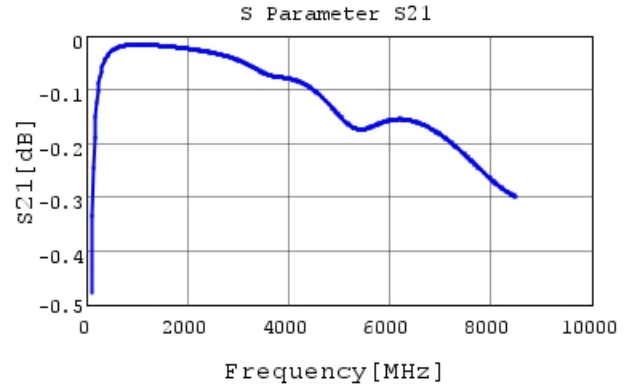
GRM0335C1H470JA01 S21 DCOV, 25degC
