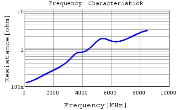
GRM0335C1H470JA01 R DCOV, 25degC
