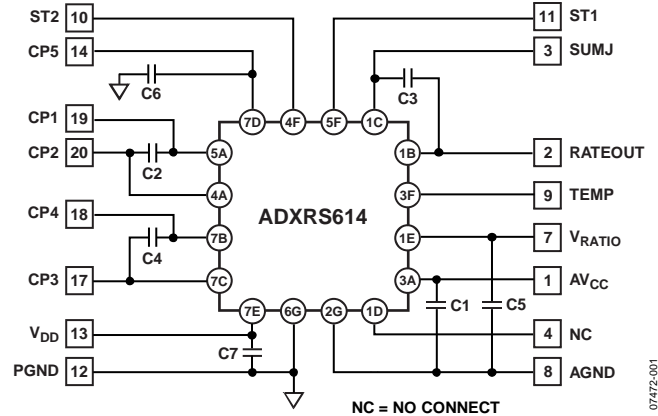
Figure 1. EVAL-ADXRS614 Schematic
