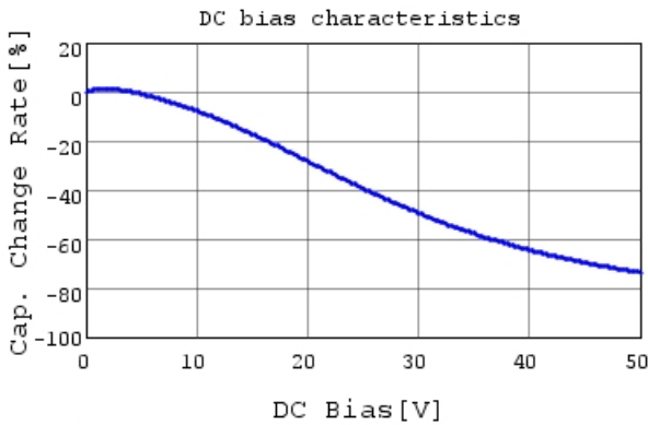
GCM32EC71H106KA03 C-DC bias capchange, 25.0c
