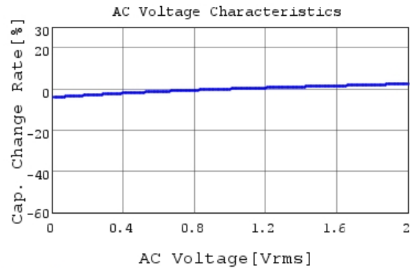
GCM32EC71H106KA03 C-AC Voltage capchange, Dc
