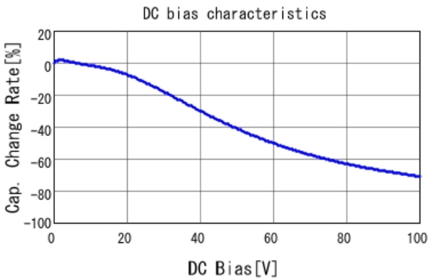
GRM31MR72A224KA01 C-DC bias capchange, 25.0degC, A
