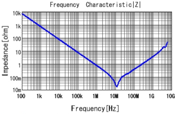
GRM31MR72A224KA01 |Z| DCOV, 25degC
