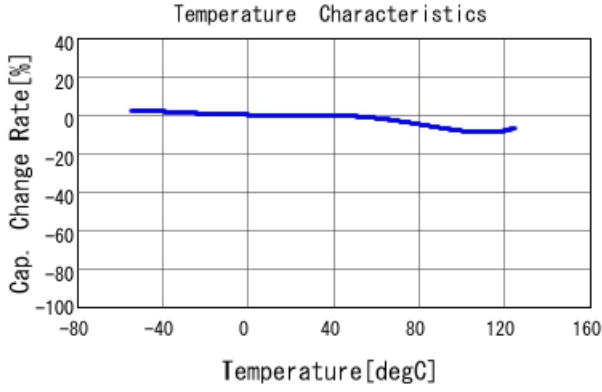
GRM31MR72A224KA01 C-Temp. capchange, DC0.0V, AC1.C
