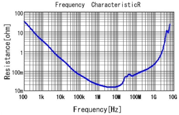
GRM31MR72A224KA01 R DCOV, 25degC
