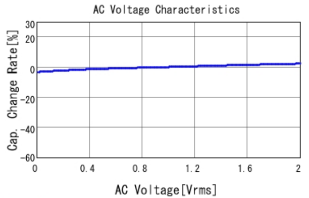
GRM31MR72A224KA01 C-AC Voltage capchange, DCOV, 25
