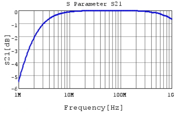
RCE5C1H102J0K1H03B S21 DC0V, 25degC
