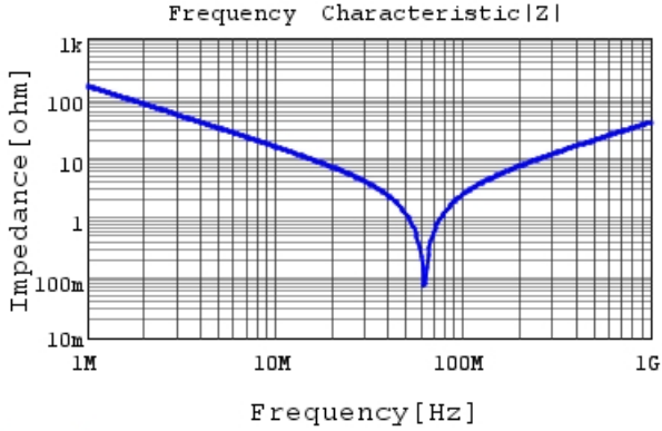
RCE5C1H102J0K1H03B |Z| DC0V, 25degC
