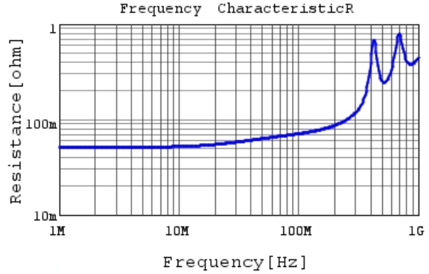
RCE5C1H102J0K1H03B R DC0V, 25degC
