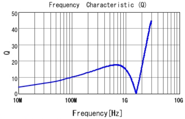
LQG15HN47NJ02 Q
