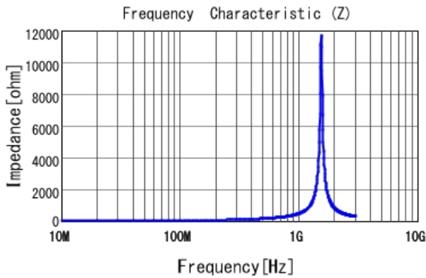
LQG15HN47NJ02 |Z|
