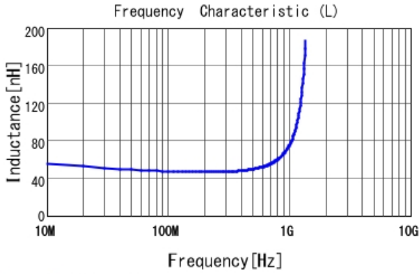
LQG15HN47NJ02 L
