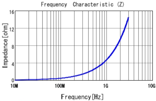
LQP03HQ0N7W02 |Z|
