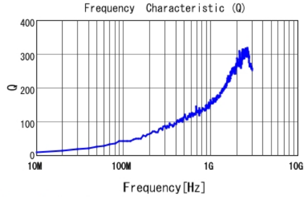
LQP03HQ0N7W02 Q
