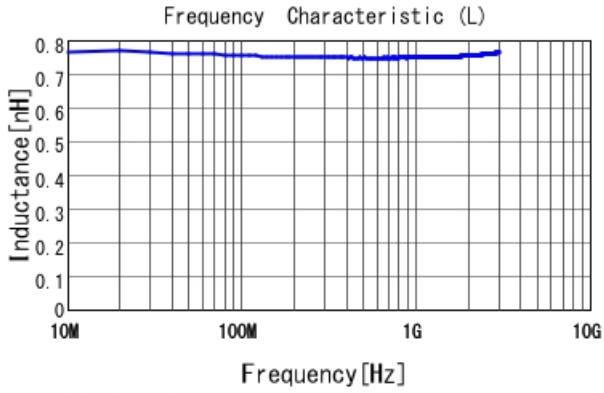
LQP03HQ0N7W02 L
