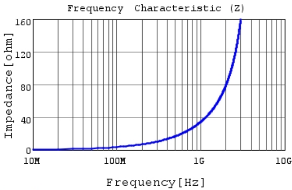
LQG15HS5N6S02 |Z|
