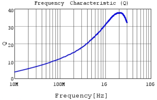
LQG15HS5N6S02 Q
