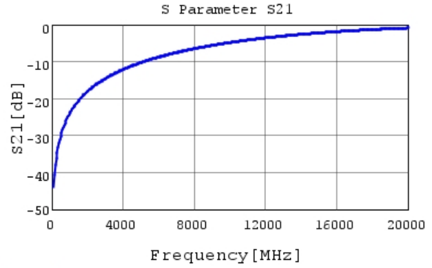
GRM0335C1HR10WA01 S21 DCOV, 25degC
