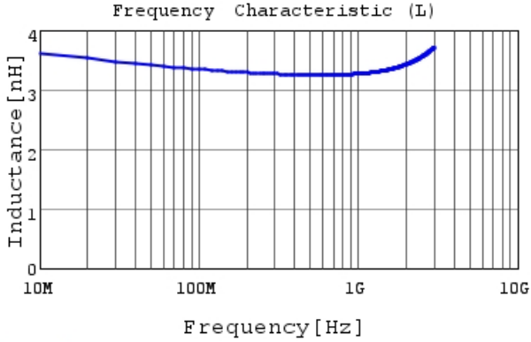
LQG15WH3N3B02 L
