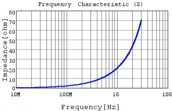
LQG15WH3N3B02 |Z|
