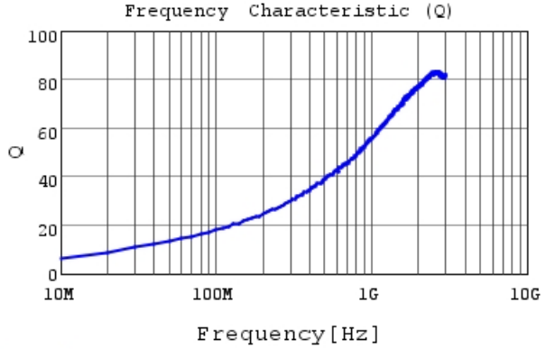
LQG15WH3N3B02 Q
