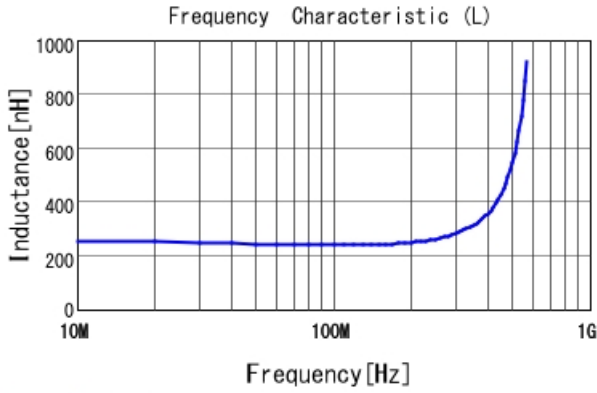
LQP03TNR24H02 L
