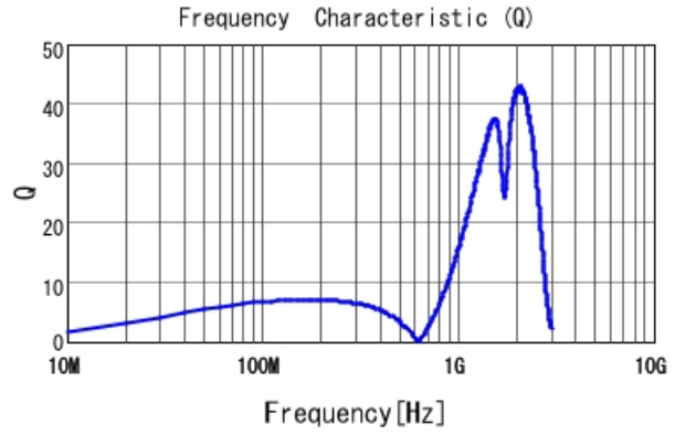
LQP03TNR24H02 Q
