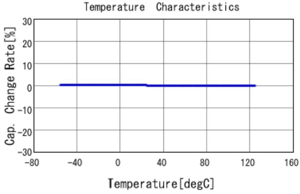
GRM1555C1H122JA01 C-Temp. capchange, DCOV, AC1Vrms
