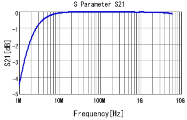
GRM1555C1H122JA01 S21 DCOV, 25degC
