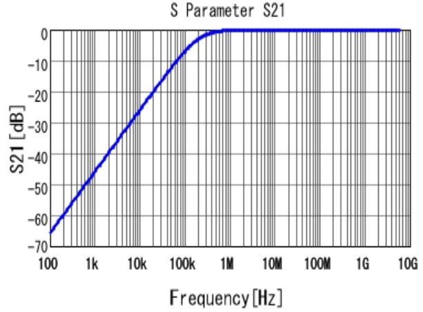
■ GRM155R71E822KA01 S21 DCOV, 25degC
