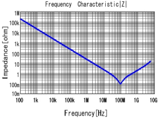
■ GRM155R71E822KA01 |Z| DCOV, 25degC
