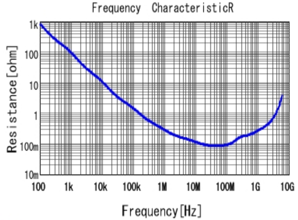
■ GRM155R71E822KA01 R DCOV, 25degC
