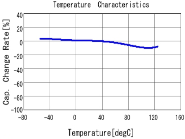
■ GRM155R71E822KA01 C-Temp. capchange, DCO. 0V, AC1.0V rm
