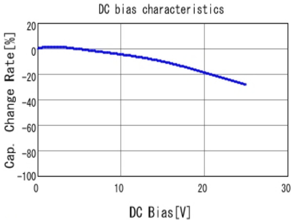
■ GRM155R71E822KA01 C-DC bias capchange, 25.0degC, AC1.
