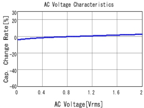
■ GRM155R71E822KA01 C-AC Voltage capchange, DCOV, 25.0d
