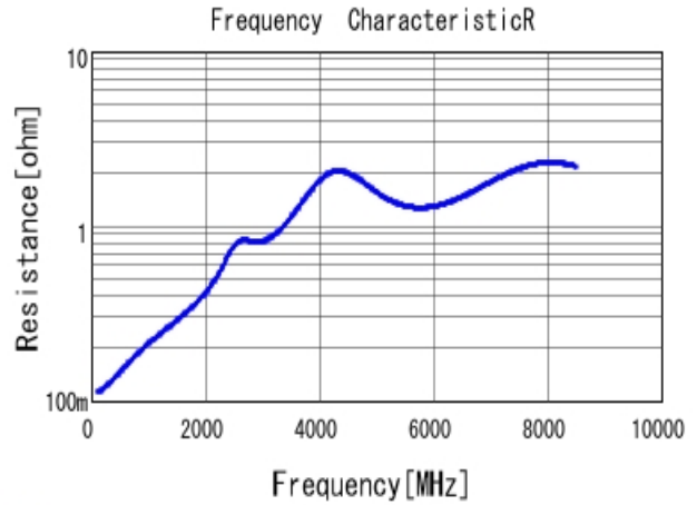
■ GRM1555C1H680JA01 R DCOV, 25degC
