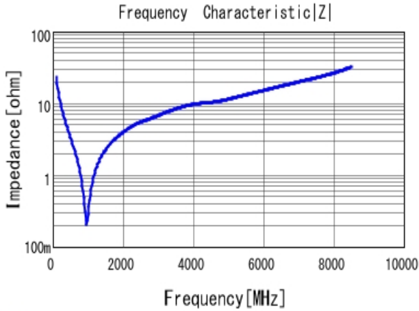
■ GRM1555C1H680JA01 |Z| DCOV, 25degC
