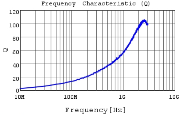
LQG15WH1N8B02 Q
