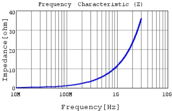
LQG15WH1N8B02 |Z|
