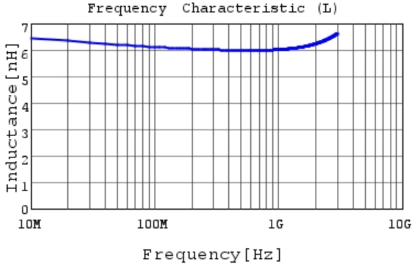
LQW15AN6N2D00 L
