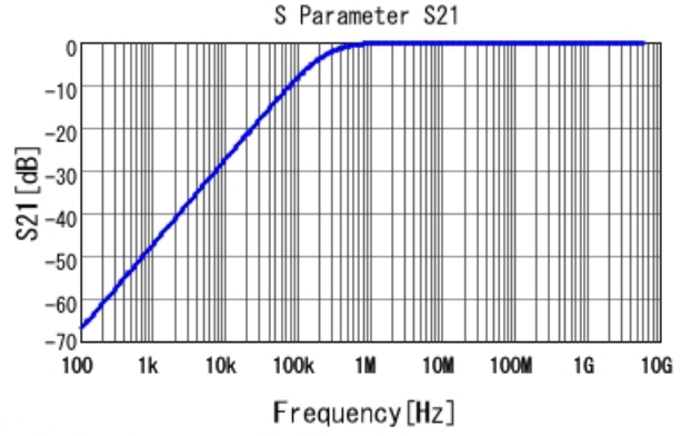
■ GRM033R71E682KE14 S21 DCOV, 25degC
