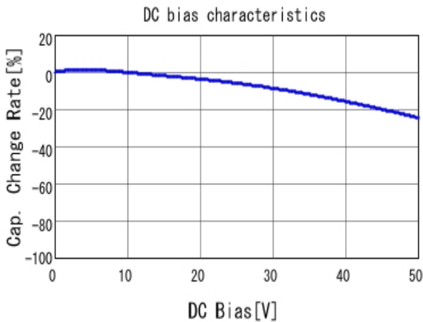
■ GRM155R71H471KA01 C-DC bias capchange, 25.0degC, AC1.
