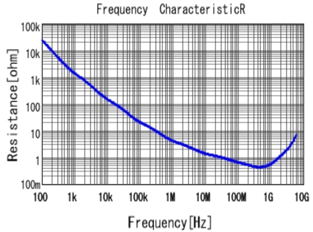
■ GRM155R71H471KA01 R DCOV, 25degC
