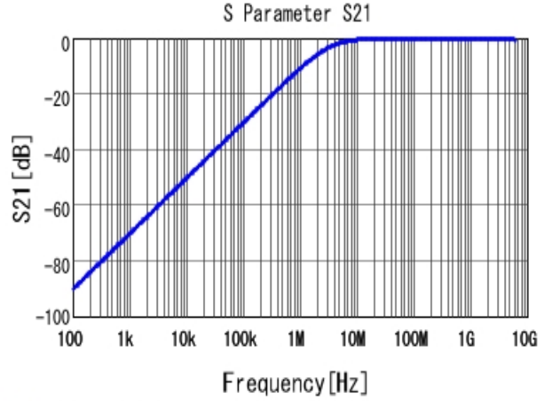
■ GRM155R71H471KA01 S21 DCOV, 25degC
