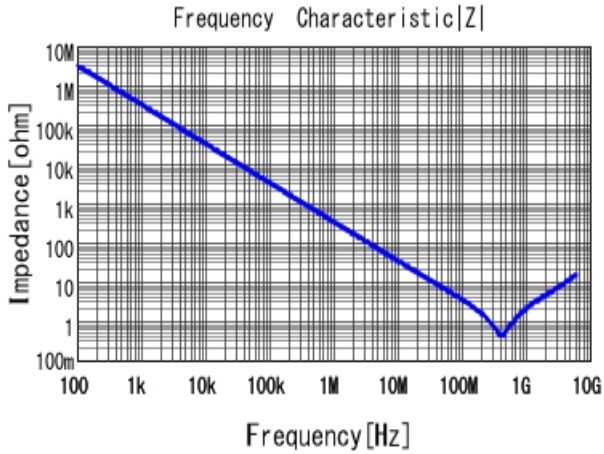
■ GRM155R71H471KA01 |Z| DCOV, 25degC
