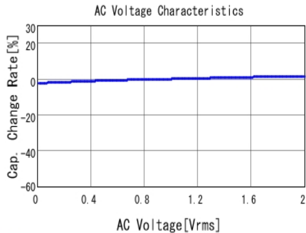
■ GRM155R71H471KA01 C-AC Voltage capchange, DCOV, 25.0d
