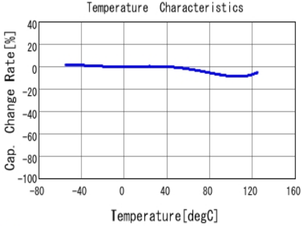
■ GRM155R71H471KA01 C-Temp. capchange, DCO. 0V, AC1.0Vrm
