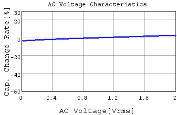
GCM155R71H223KA55 C-AC Voltage capchange, DC
