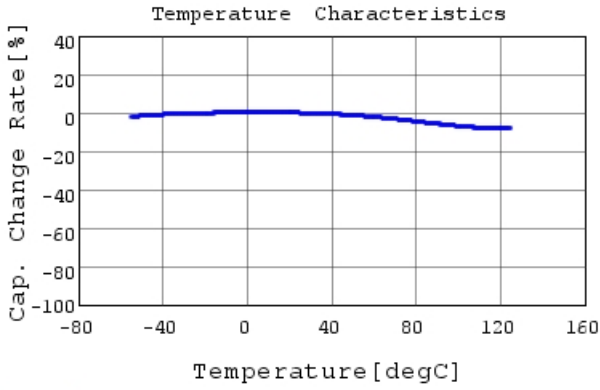
GCM155R71H223KA55 C-Temp. capchange, DC0.0V,
