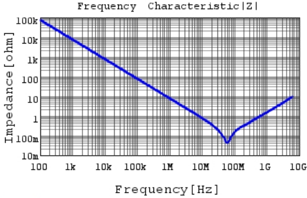
GCM155R71H223KA55 |Z| DC0V, 25degC
