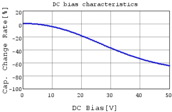
GCM155R71H223KA55 C-DC bias capchange, 25.0c
