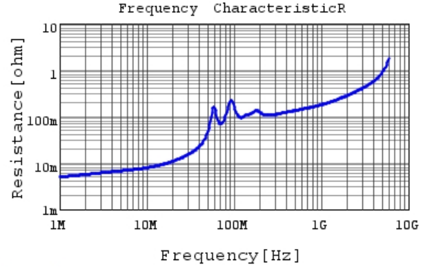
GRM3195C1H473JA05 R DC0V, 25degC
