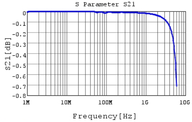
GRM3195C1H473JA05 S21 DCOV, 25degC
