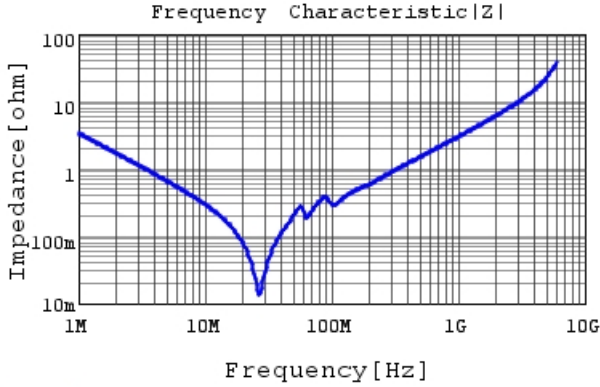
GRM3195C1H473JA05 |Z| DC0V, 25degC
