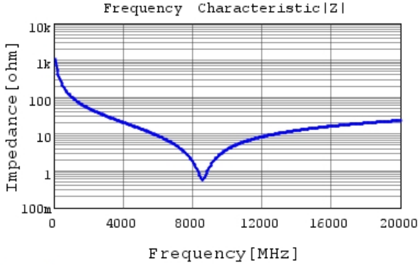
GRM0225C1H1R5WA03 |Z| DC0V, 25degC
