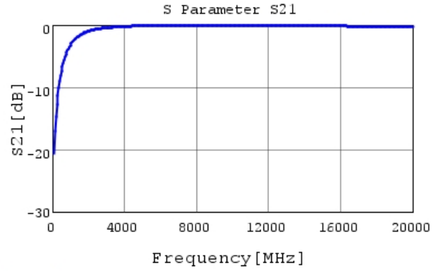
GRM0225C1H1R5WA03 S21 DCOV, 25degC
