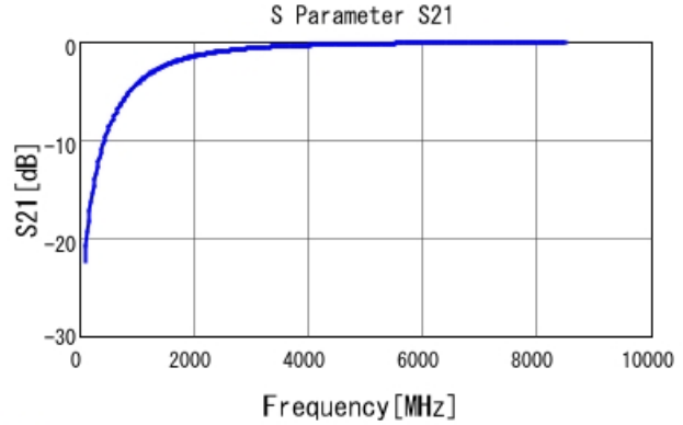
■ GRM0335C1H1R2BA01 S21 DCOV, 25degC
