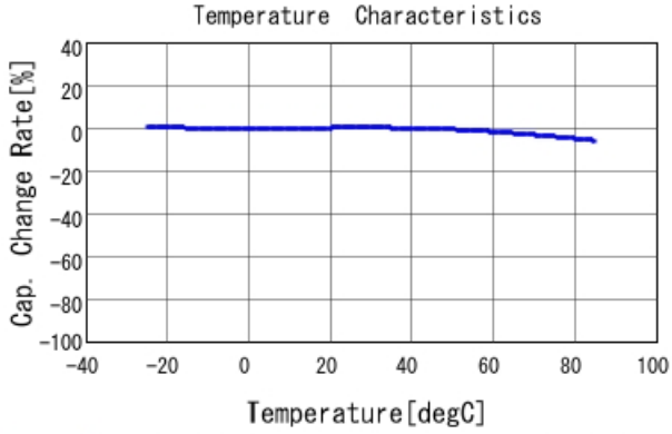
GRM15XB11E222KA86 C-Temp. capchange, DC0.0V, AC1.C
