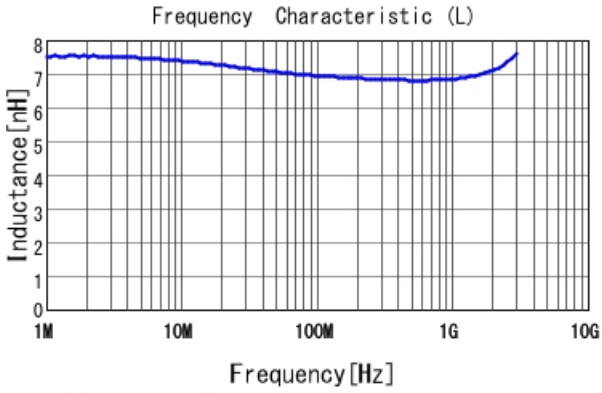
LQW15AN7N0G8Z L
