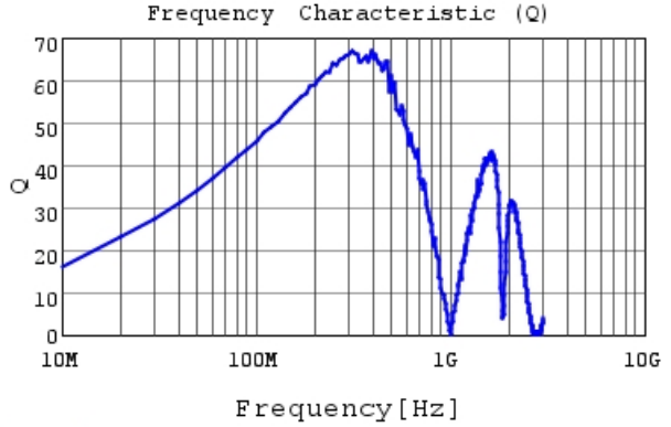
LQW2BASR22G00 Q
