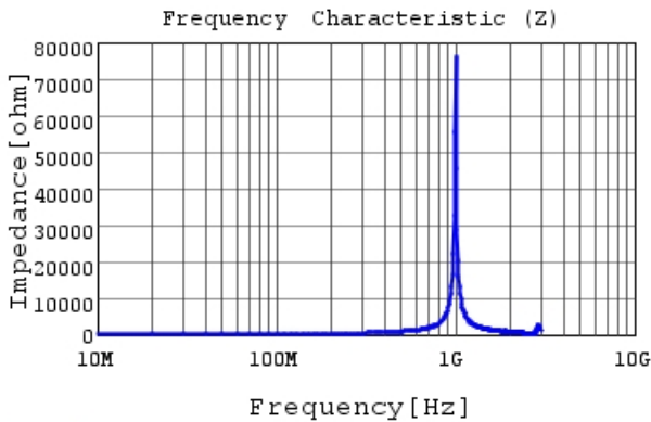
LQW2BASR22G00 |Z|
