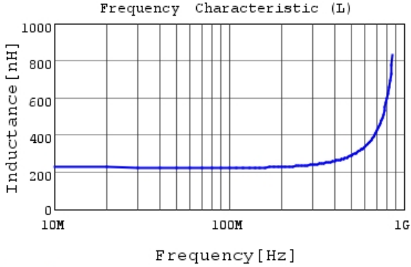
LQW2BASR22G00 L
