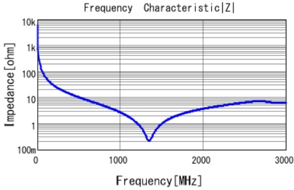
GRM1885C2E270JW07 |Z| DCOV, 25degC
