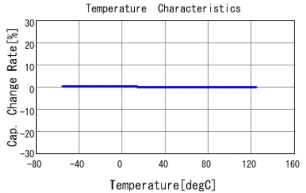
GRM1885C2E270JW07 C-Temp. capchange, DCOV, AC1Vrms
