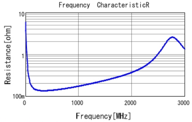
GRM1885C2E270JW07 R DCOV, 25degC
