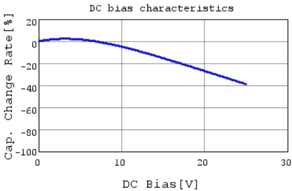
KRM55WR71E476MH01 C-DC bias capchange, 25.0c
