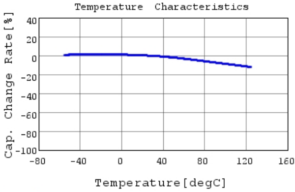
KRM55WR71E476MH01 C-Temp. capchange, DCOV, 1
