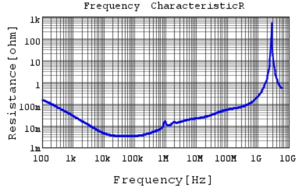
KRM55WR71E476MH01 R DCOV, 25degC
