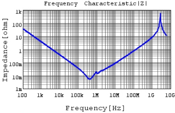
KRM55WR71E476MH01 |Z| DCOV, 25degC
