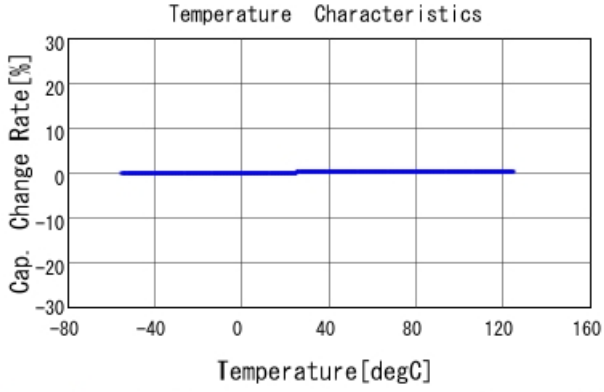
GJM1555C1H1R8WB01 C-Temp. capchange, DCOV, AC1Vrms
