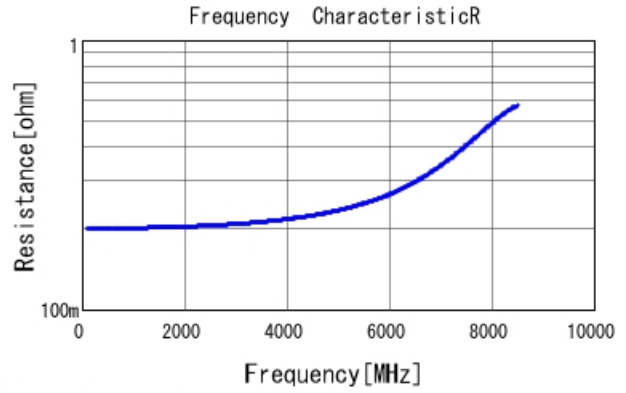
GJM1555C1H1R8WB01 R DCOV, 25degC
