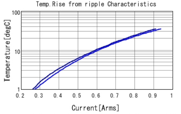
GJM1555C1H1R8WB01 Temp. rise — 2GHz — 3GHz
