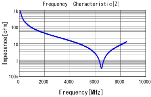
GJM1555C1H1R8WB01 |Z| DCOV, 25degC
