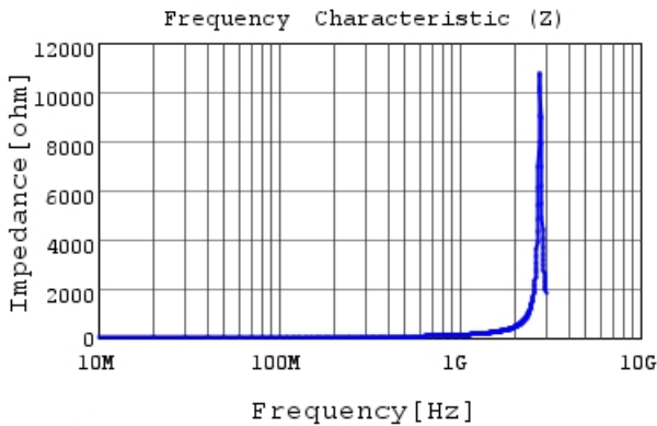
LQG15HS18NJ02 |Z|
