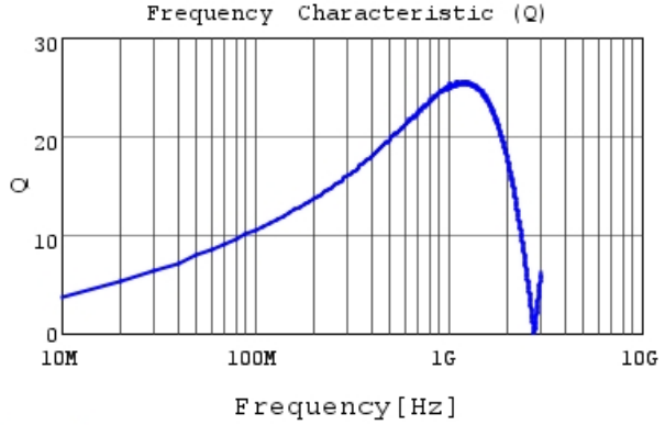
LQG15HS18NJ02 Q
