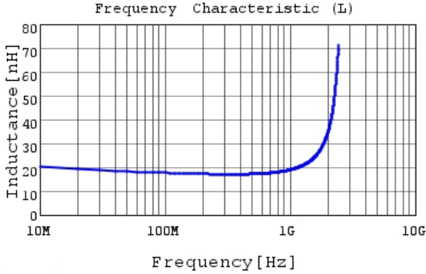
LQG15HS18NJ02 L
