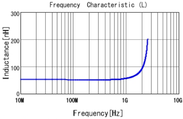
LQW15AW51NJ80 L
