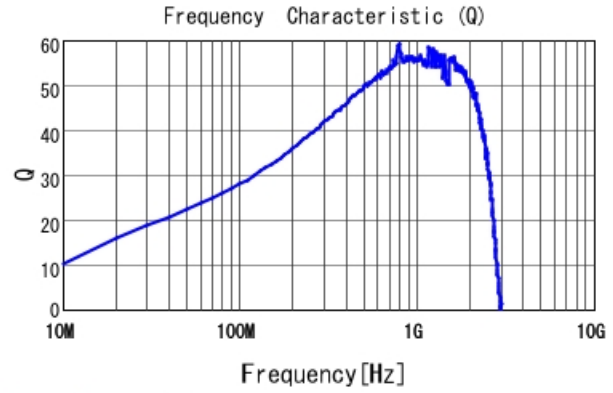
LQW15AW51NJ80 Q
