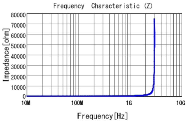
LQW15AW51NJ80 |Z|
